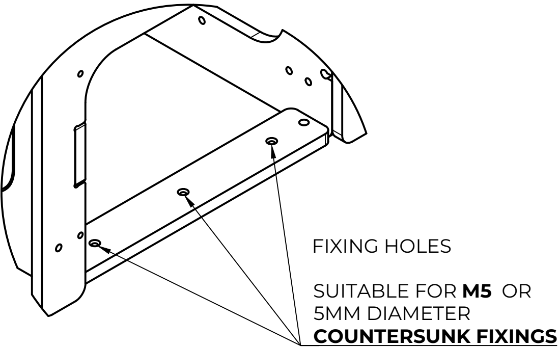
VIEW A
