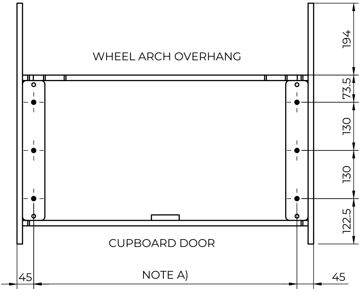
TOP VIEW SHOWN WITH BED SLATS REMOVED
